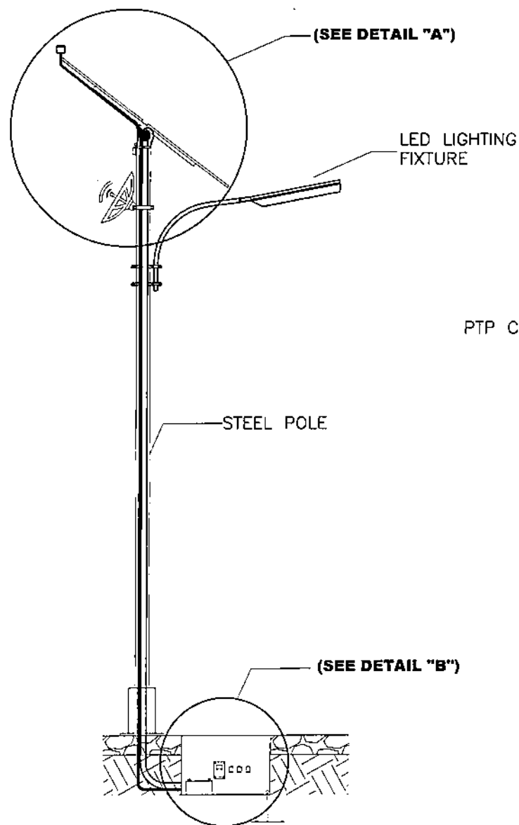
STRONG MOTION ACCELEROMETER INSTALLATION DETAILS
