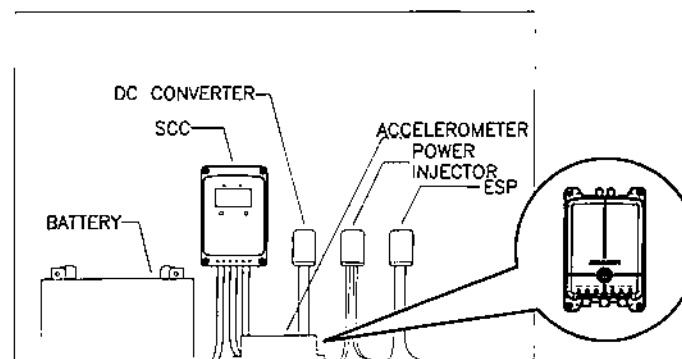
DETAIL B
